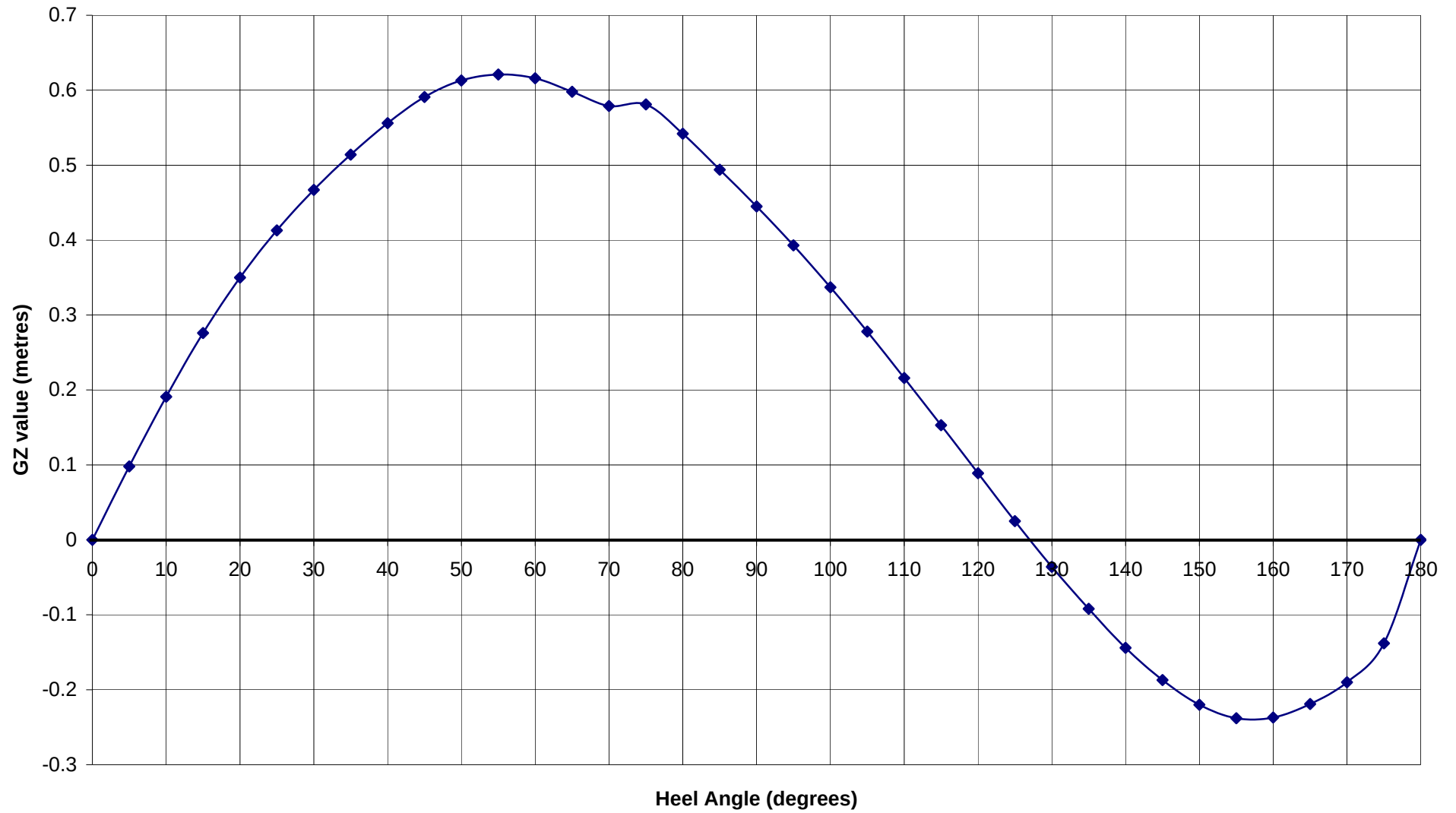
Elan 410 Preliminary GZ Curve
